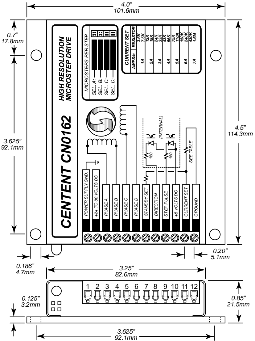
Figure 1: CN0162 MICROSTEP DRIVE (Actual Size)
