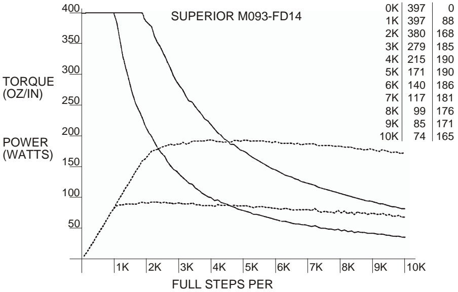
Figure 15 - SUPERIOR M093-FD14
