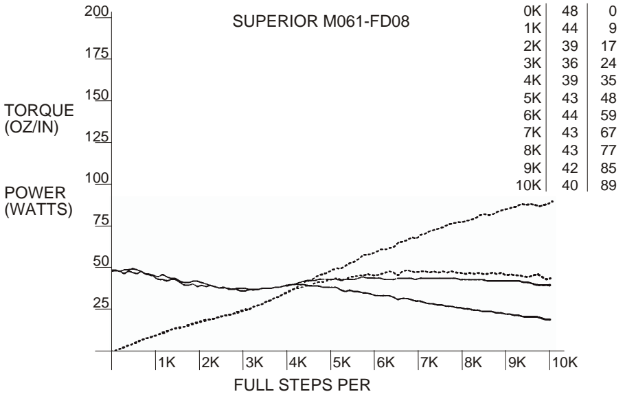
Figure 32 - SUPERIOR M061-FD08
