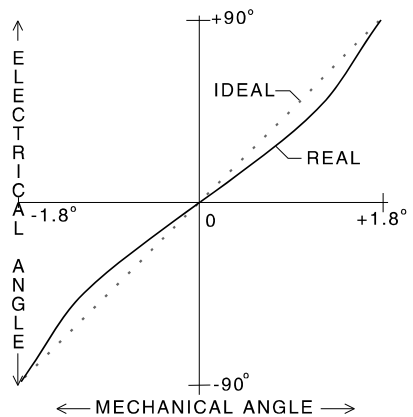
Figure 14 - Motor linearity
