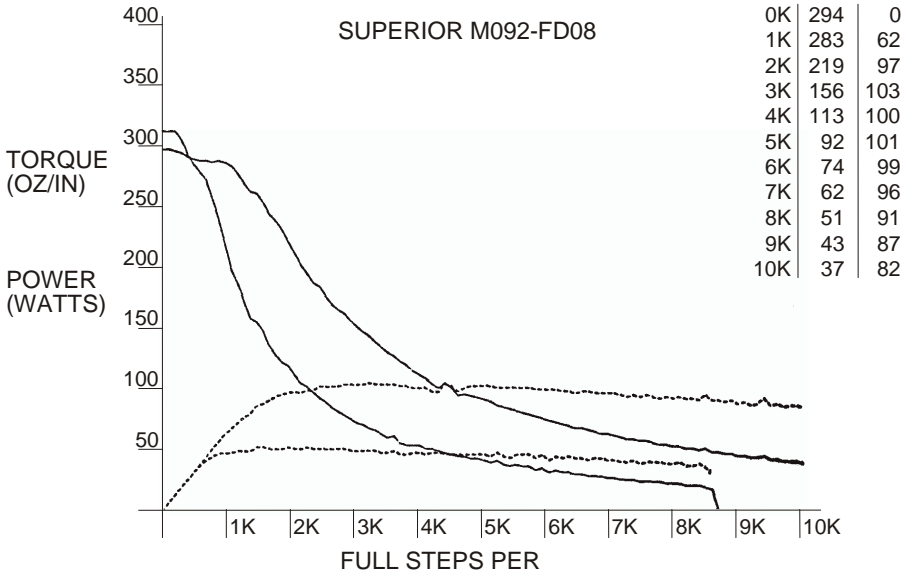
Figure 27 - SUPERIOR M092-FD08
