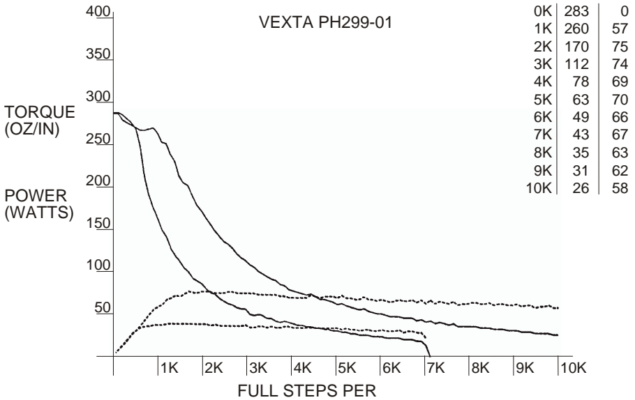
Figure 36 - VEXTA PH299-01
