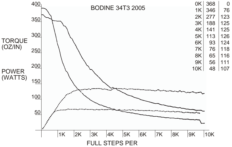
Figure 21 - BODINE 34T3 2005
