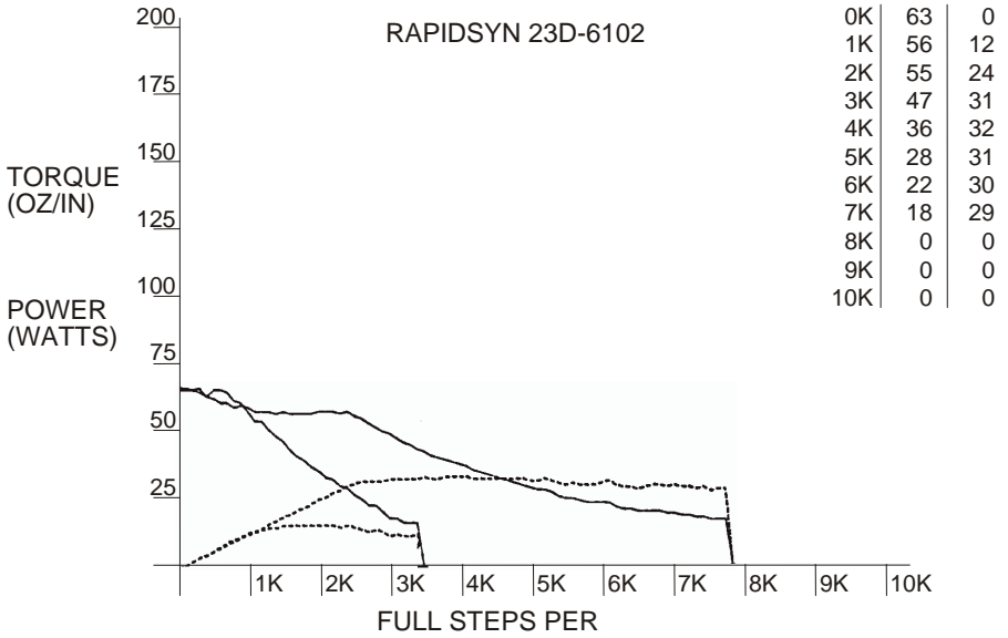
Figure 41 - RAPIDSYN 23D-6102
