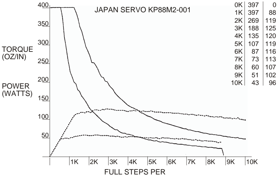
Figure 22 - JAPAN SERVO KP88M2-001
