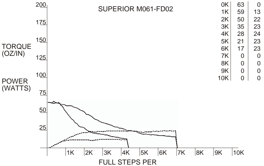
Figure 42 - SUPERIOR M061-FD02
