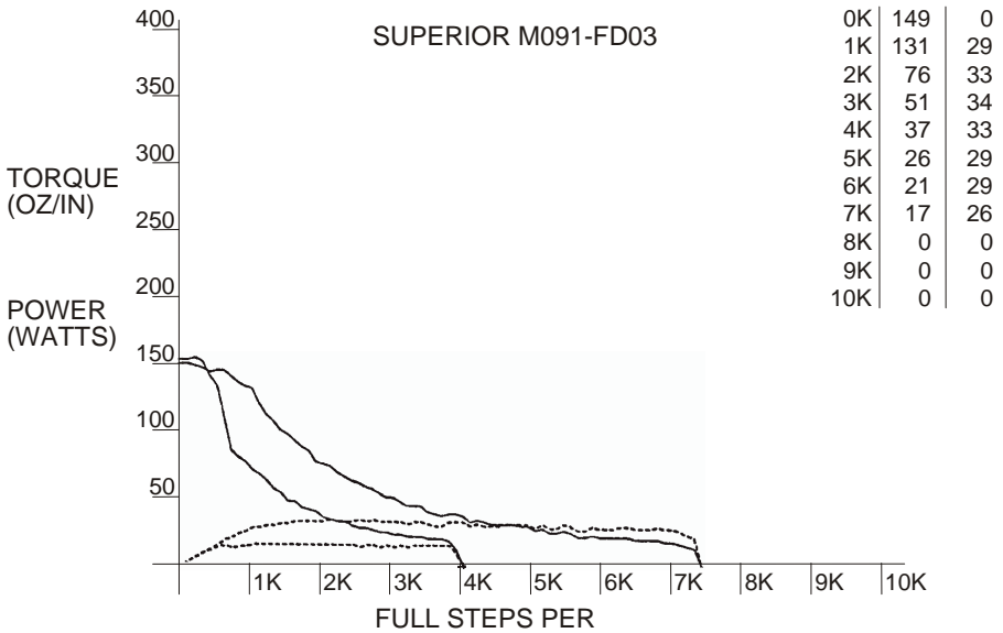
Figure 40 - SUPERIOR M091-FD03
