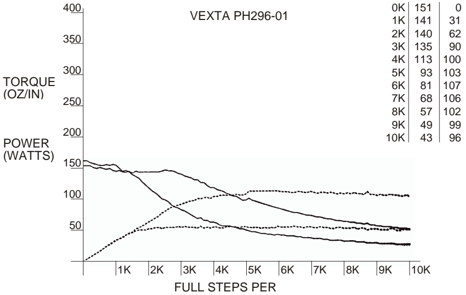
Figure 25 - VEXTA PH296-01
