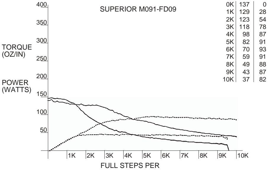
Figure 31 - SUPERIOR M091-FD09
