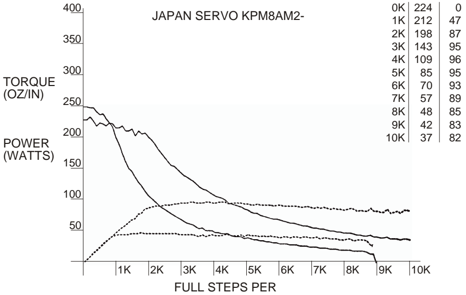
Figure 29 - JAPAN SERVO KPM8AM2-001
