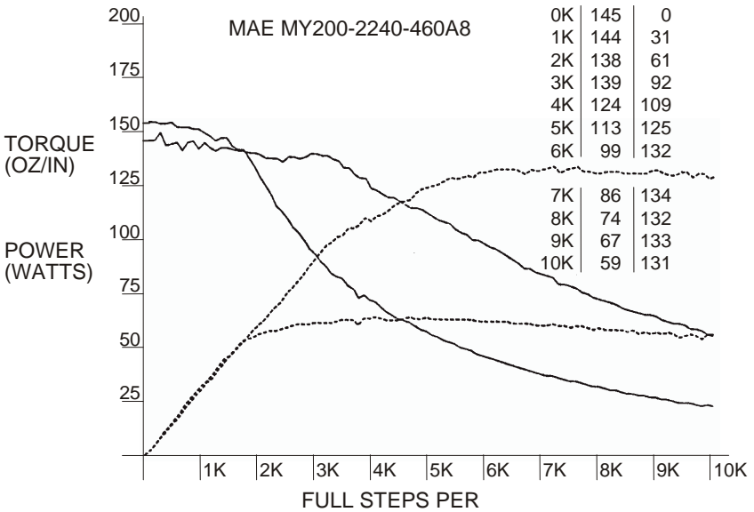
Figure 18 - MAE MY200-2240-460A8
