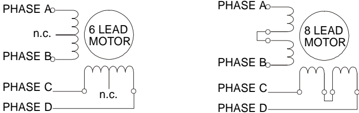
Figure 5 - Series configuration
