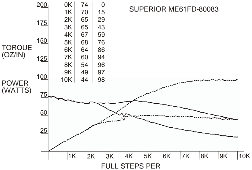
Figure 28 - SUPERIOR ME61FD-80083
