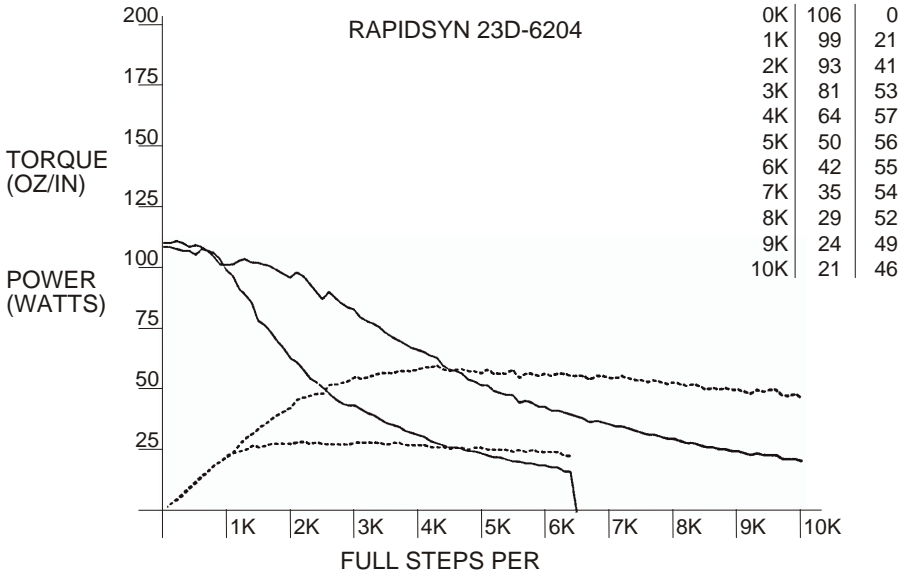
Figure 37 - RAPIDSYN 23D-6204
