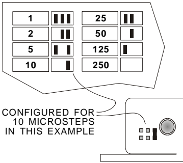
Figure 7 - Resolution Header
