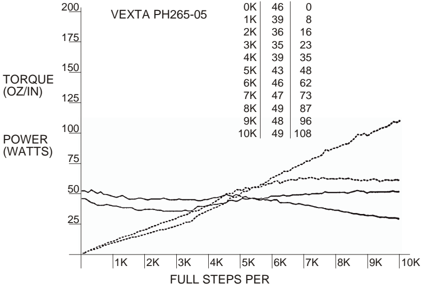
Figure 24 - VEXTA PH265-05
