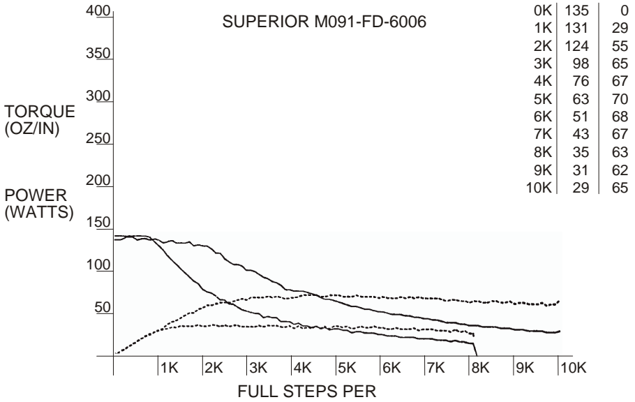
Figure 35 - SUPERIOR M091-FD-6006
