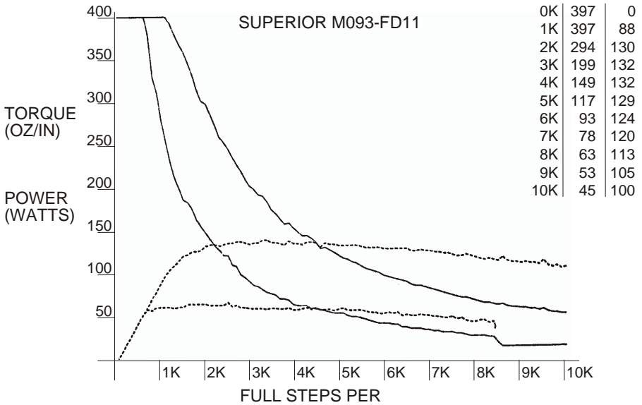
Figure 20 - SUPERIOR M093-FD11
