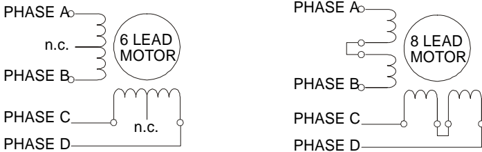
Figure 5 - Series configuration
