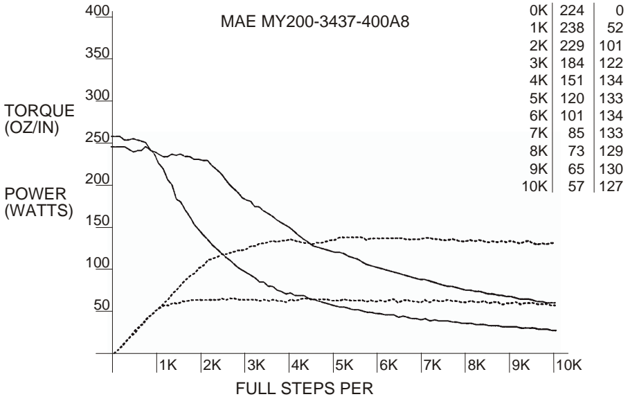
Figure 19 - MAE MY200-3437-400A8
