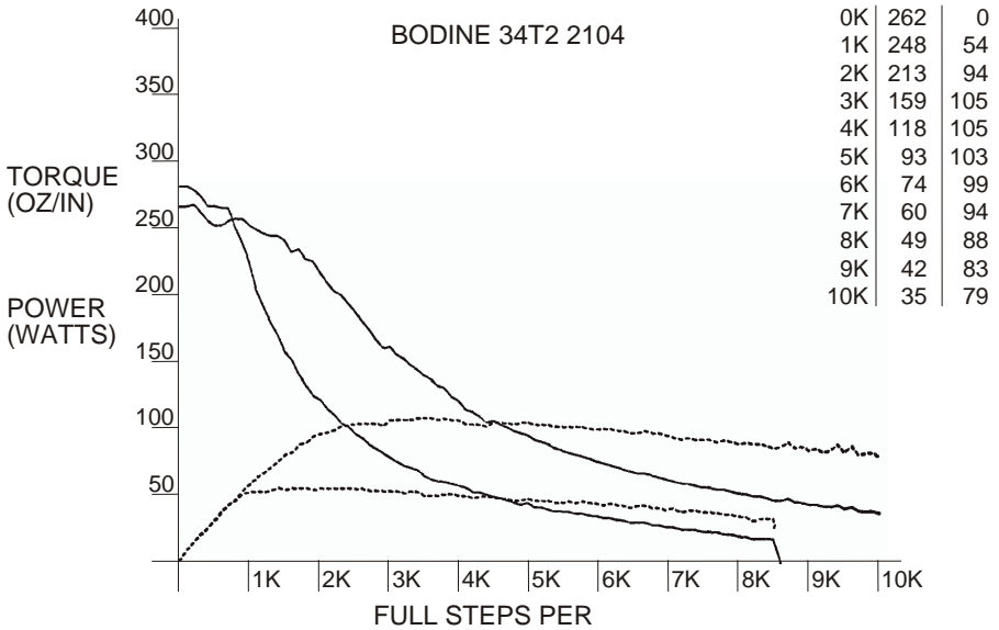
Figure 26 - BODINE 34T2 2104
