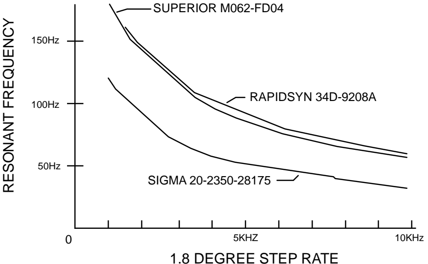
Figure 8 - Resonance
