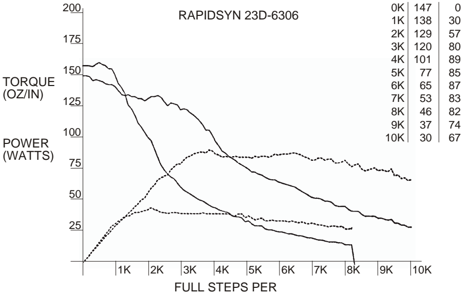
Figure 33 - RAPIDSYN 23D-6306
