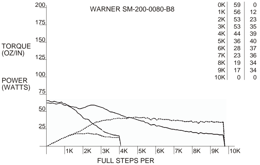
Figure 39 - WARNER SM-200-0080-B8
