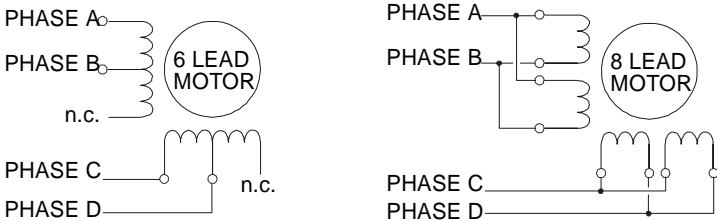
Figure 4 - Parallel configuration
