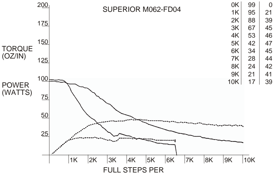
Figure 38 - SUPERIOR M062-FD04
