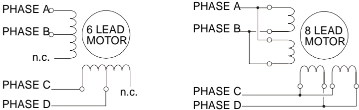
Figure 4 - Parallel configuration
