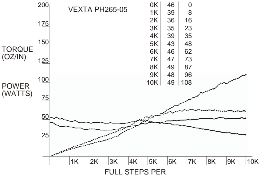
Figure 24 - VEXTA PH265-05
