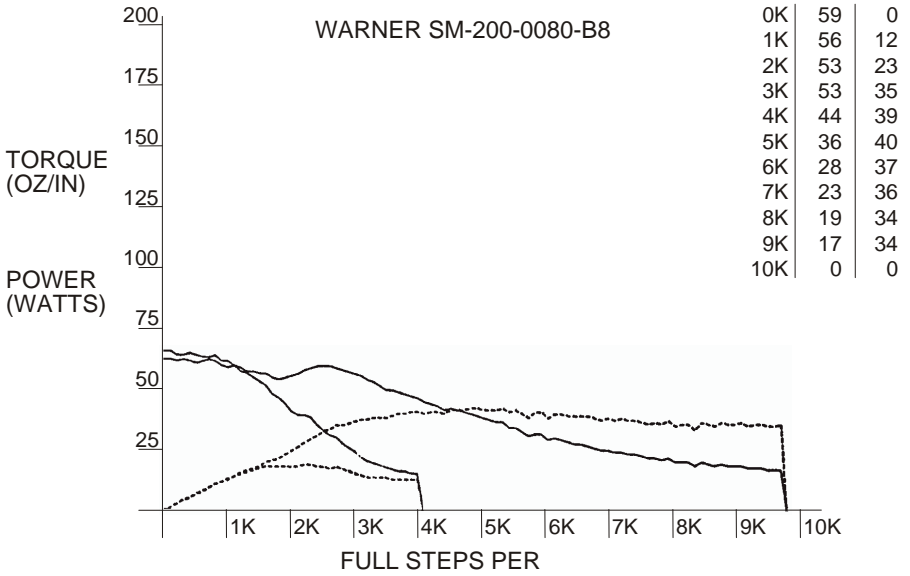
Figure 39 - WARNER SM-200-0080-B8
