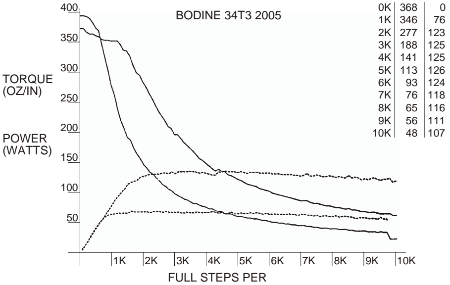
Figure 21 - BODINE 34T3 2005
